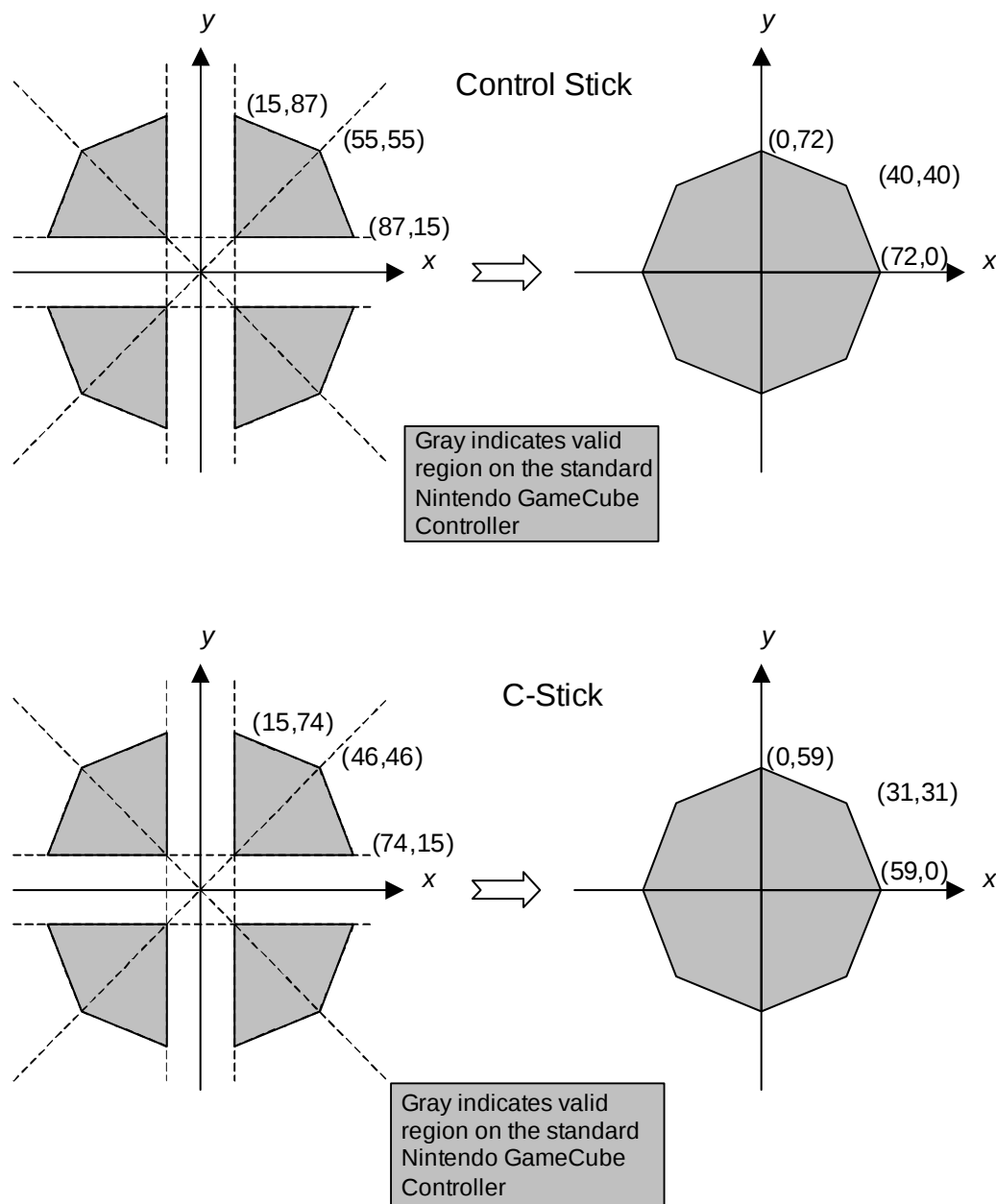
Figure 2–1 PADClamp Algorithm
