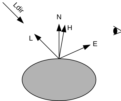
Equation 6-11 Specular Attenuation
