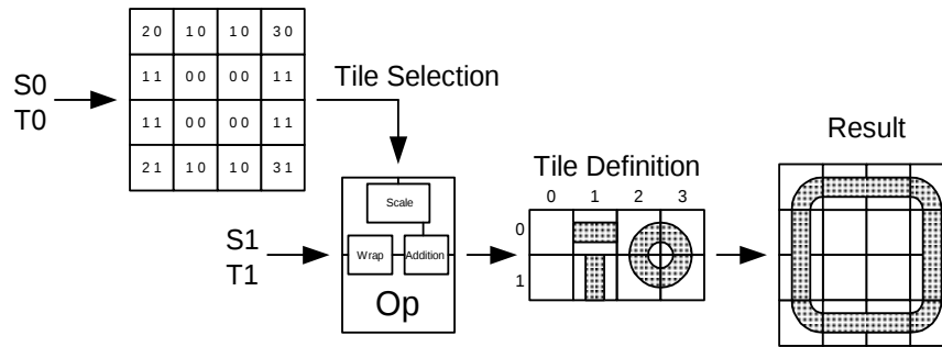
Figure 6–1 Tile Texture
