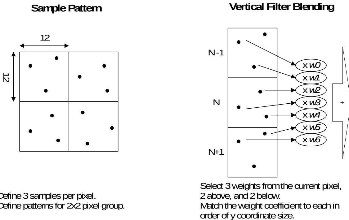
Figure 14–1 Antialiasing
