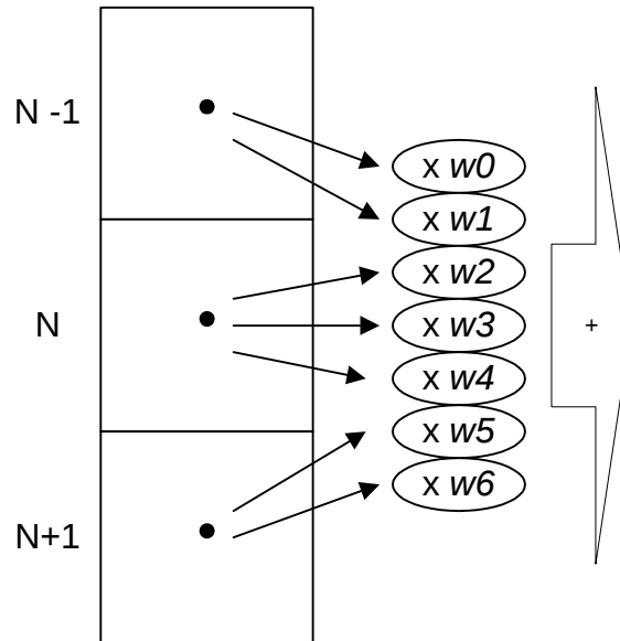
Figure 14–2 Non-antialiasing Blending
