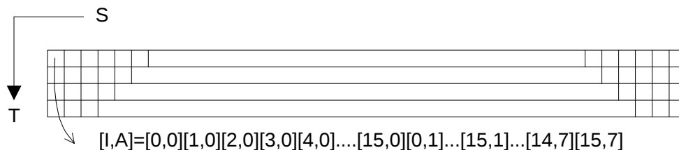
Indirect Texture
