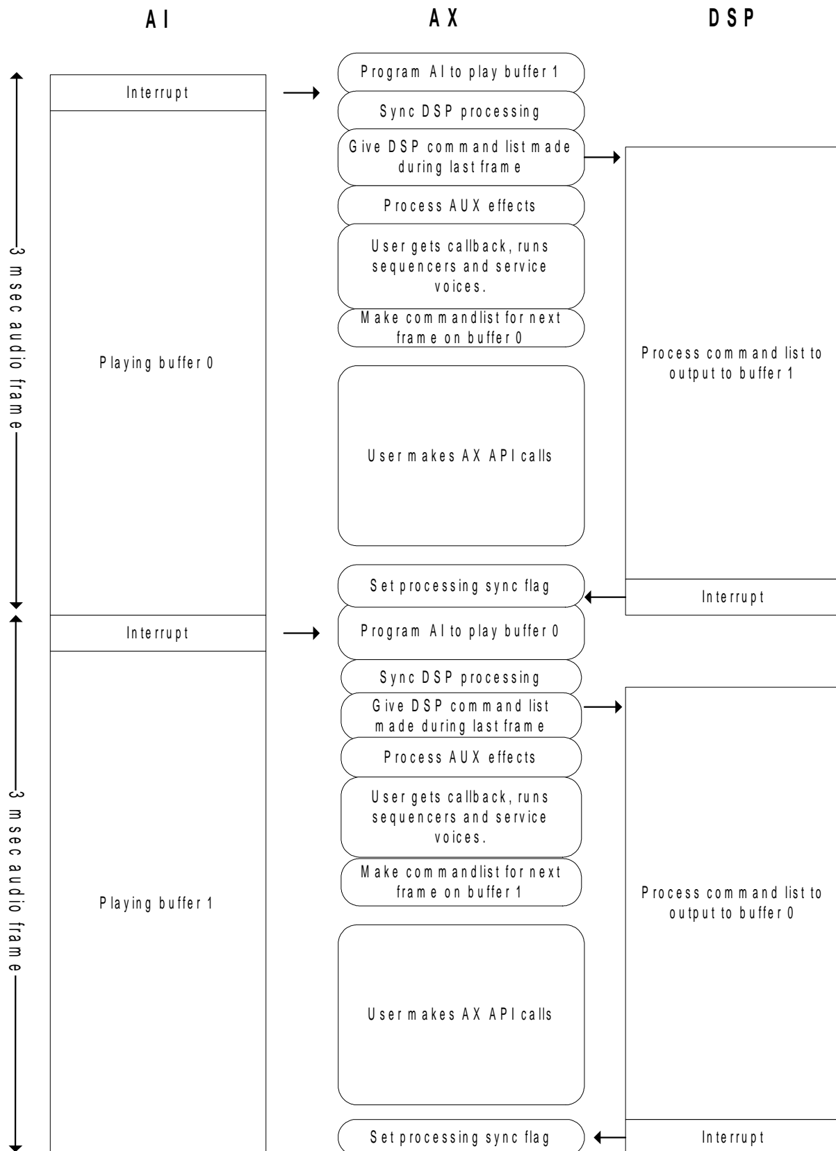
Figure 2–1 AX Library Logical Flow
