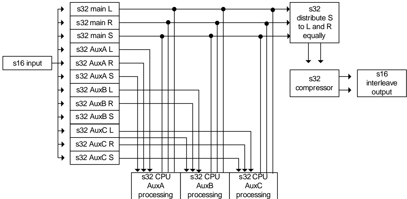
Figure 2–3 Stereo Mixing
