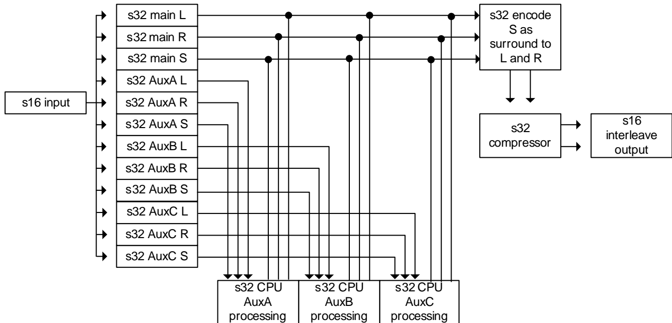
Figure 2-4 Surround Mixing
