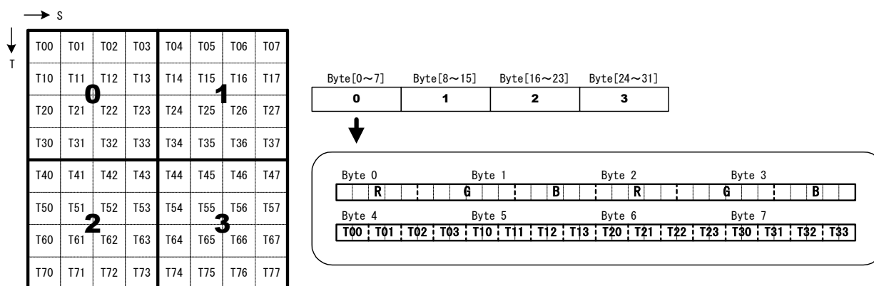
Figure 3-1 Structure of the 32-Byte Tile Requested by the Hardware
