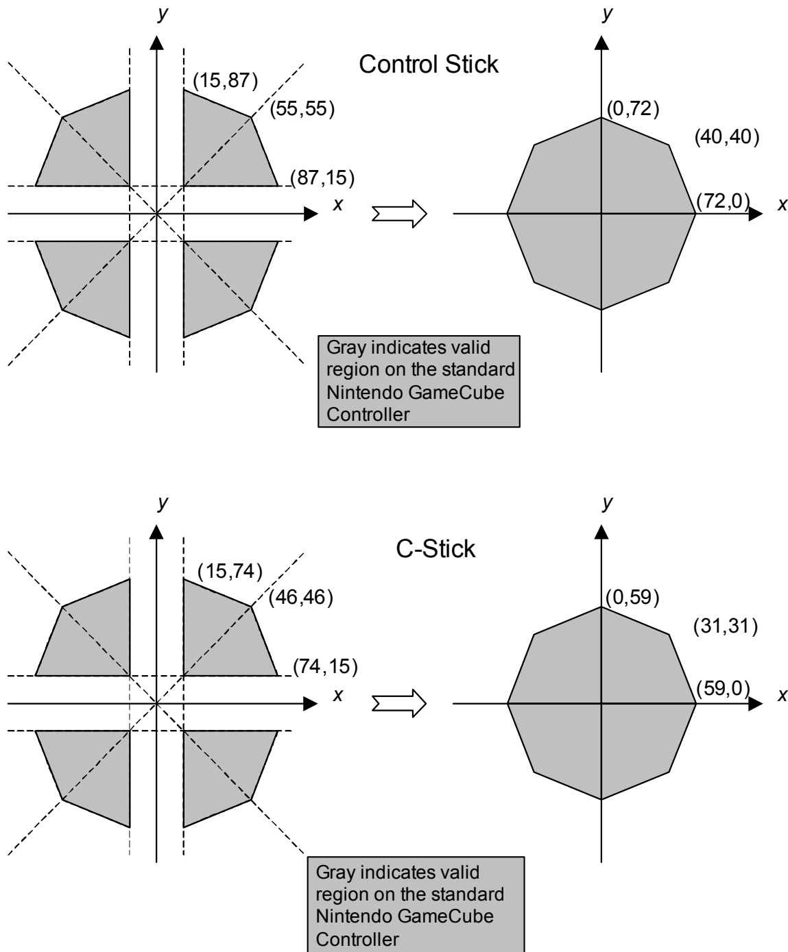
Figure 1 - PADClamp Algorithm
