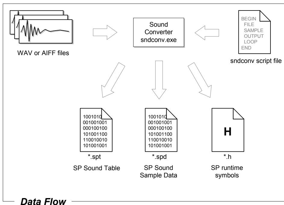
Figure 2-2 Data Flow for Importing Sound Effects
