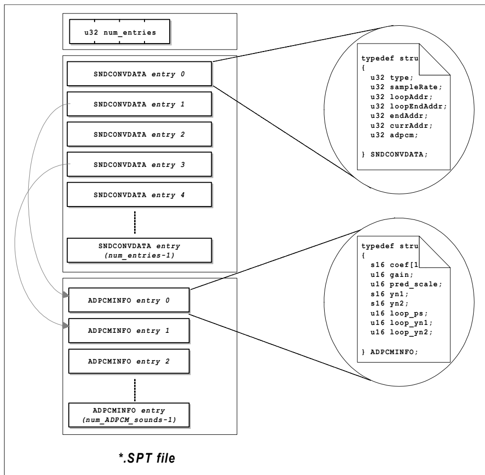
Figure 3-6 Format and Internal References of SPT Files
