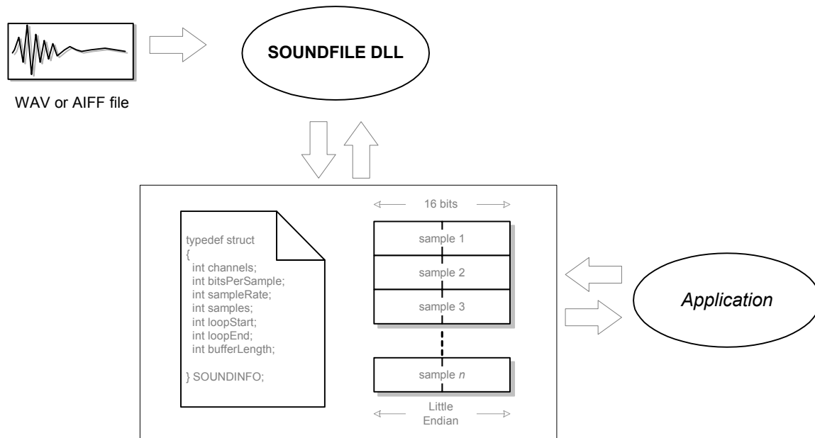
Figure 3-4 Basic Data Flow of SOUNDFILE DLL
