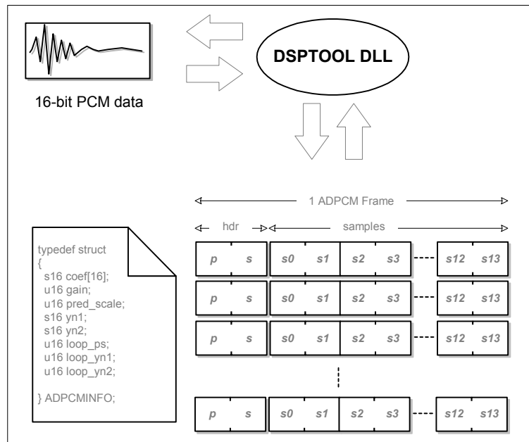
Figure 3-5 Basic Data Flow of the DSPTOOL DLL
