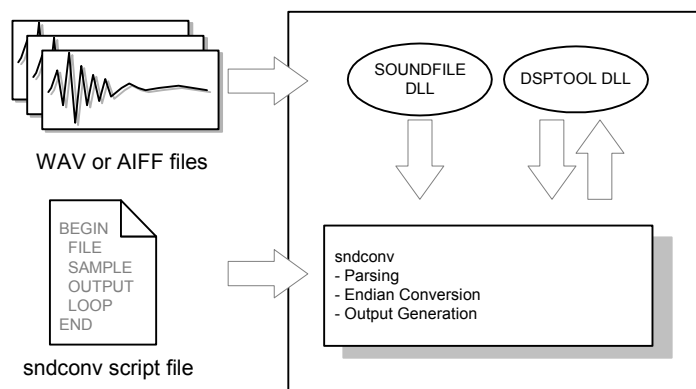
Figure 3-3 Basic Architecture and Data Flow for sndconv
