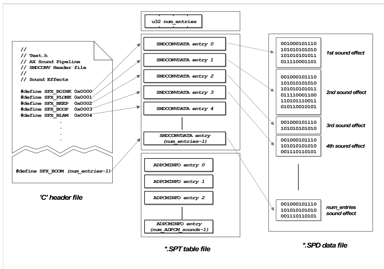
Figure 3-7 Mapping between Header File, SPT File and SPD File
