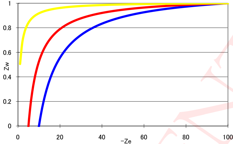
Figure 14-3: Relationship Between z_w and z_e for Different Near Values in OpenGL
