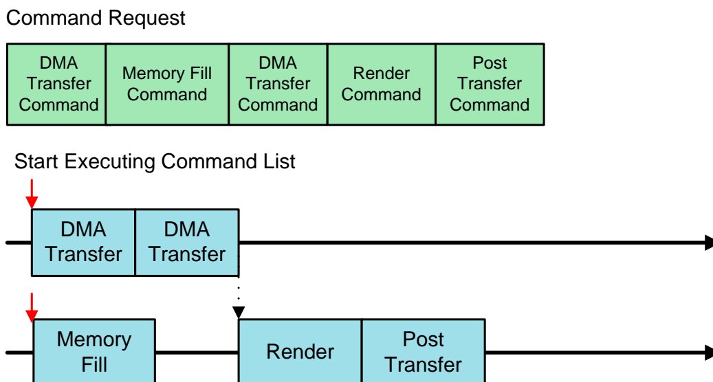
Figure 3-5 Command Execution in Synchronous Execution Mode
