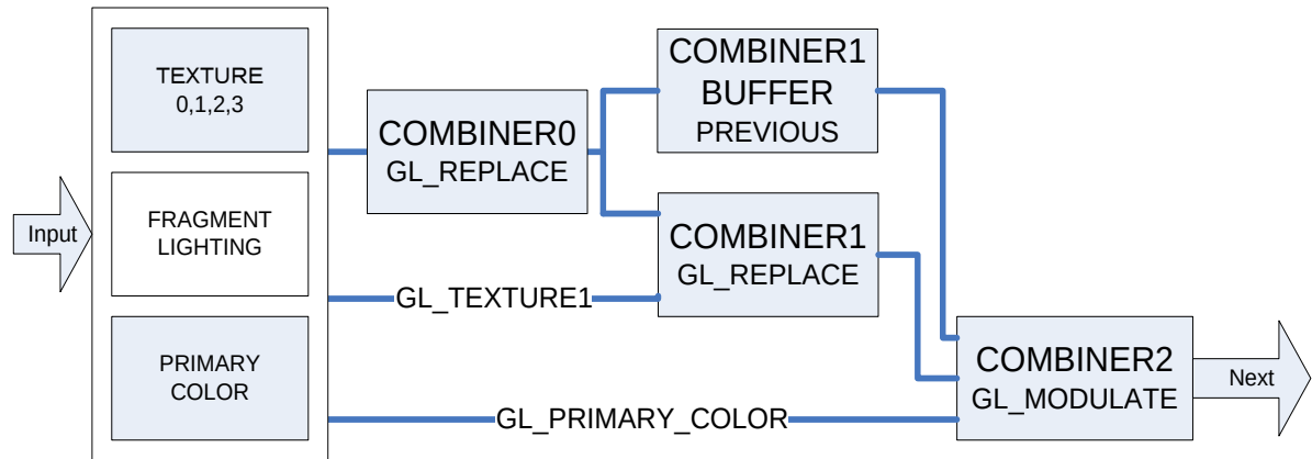
Figure 8-5: Connections Using a Previous Buffer
