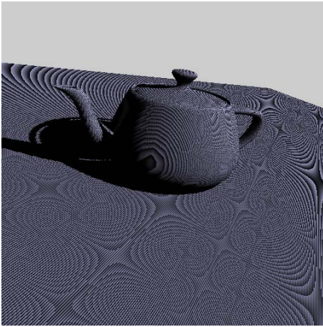
Figure 14-6: Example of Self-Shadow Aliasing
