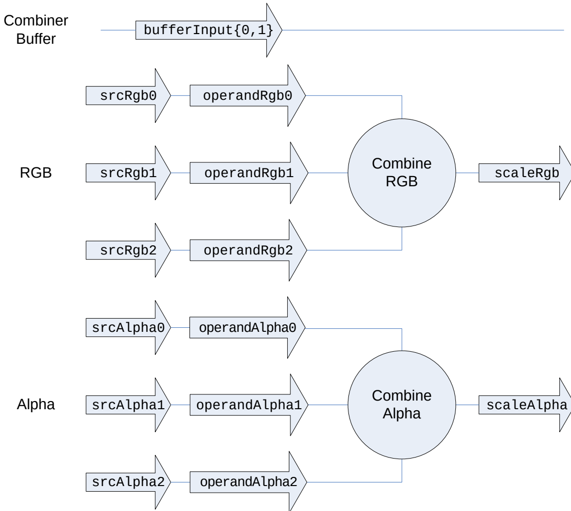
Figure 8-2: Combiner Configuration
